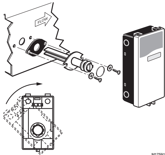
Fig. 5. Duct mounting (C7232B).
